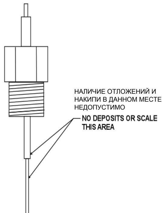
LOW WATER CUT-OFF PROBE
