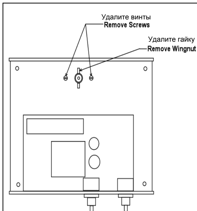
TOP VIEW OF LOW WATER CUT-OFF
